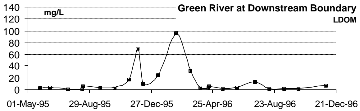
Figure 61: LDOM at Downstream Boundary: May 1995 to November 1996
