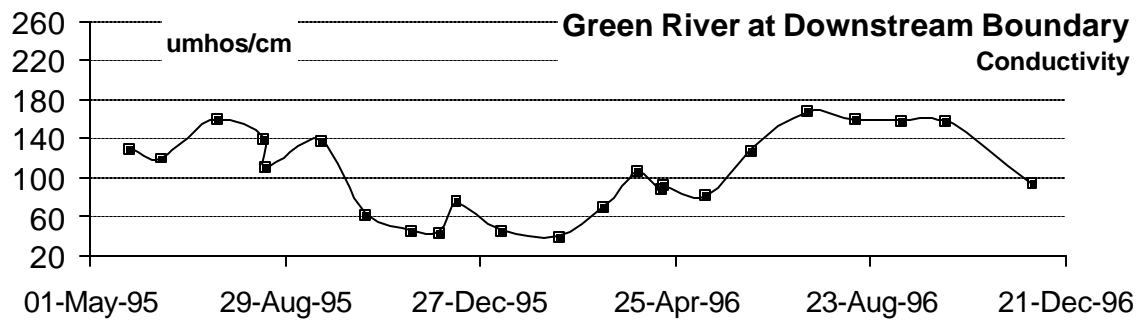
Figure 60: Conductivity at Downstream Boundary: May 1995 to November 1996
