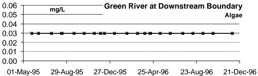
Figure 65: Algae at Downstream Boundary: May 1995 to November 1996
