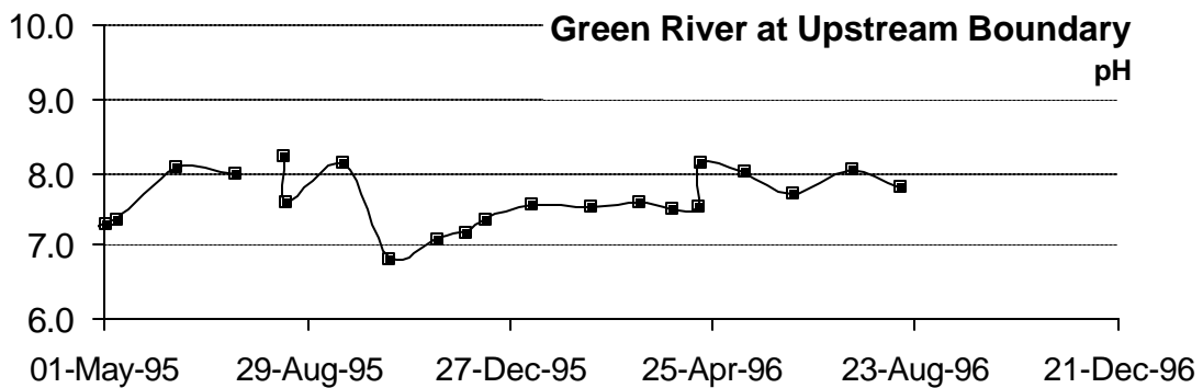
Figure 24: pH at Upstream Boundary: May 1995 to November 1996
