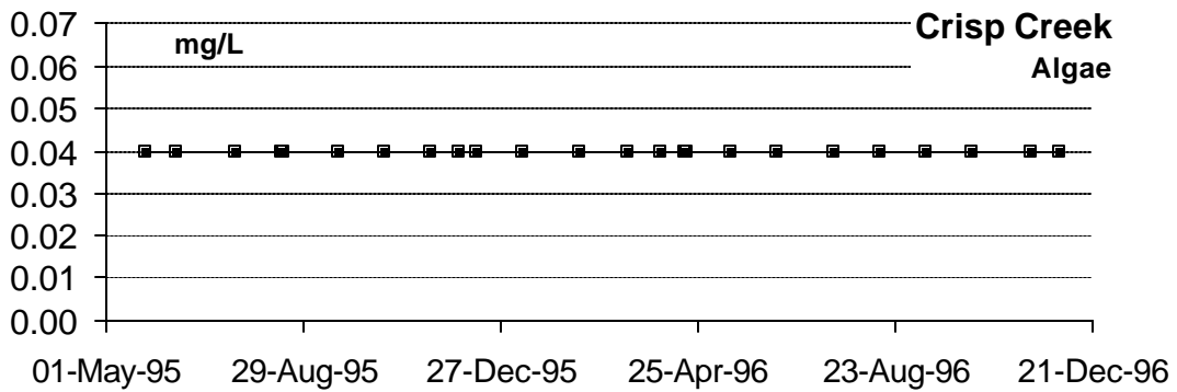
Figure 142: Algae Crisp Creek: May 25, 1995 – Nov 1996
