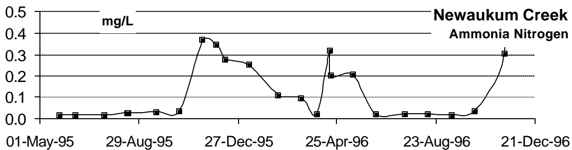
Figure 94: Ammonia Newaukum Creek: May 25, 1995 – Nov 1996
