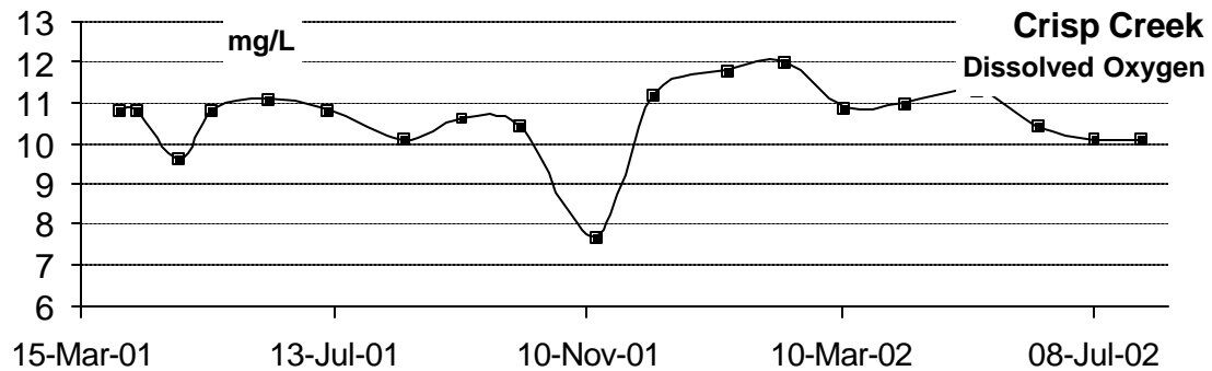
Figure 151: DO Crisp Creek: Apr 2001–July 2002
