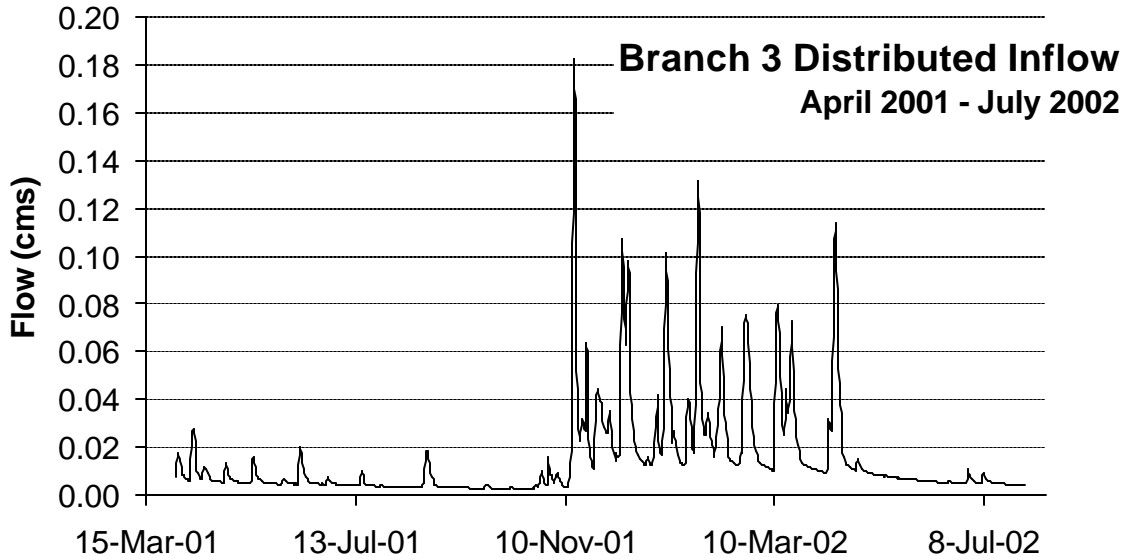
Figure 247: Branch 3 Distributed Inflow: Apr 2001 – July 2002
