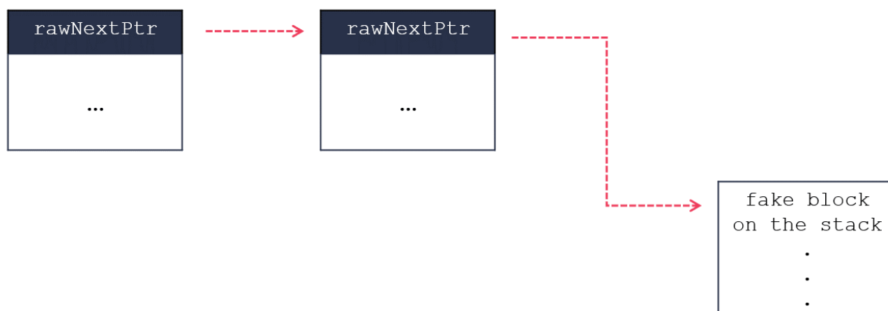
Figure 3.4: Overwriting free-list rawNextPtr pointer
