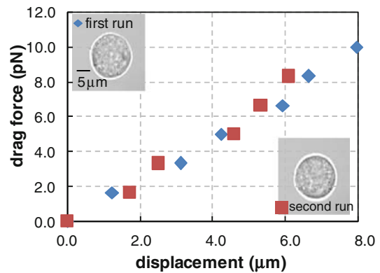
FIGURE 8. Drag force vs. displacement for a 16.5 \mu\text{m} diameter chondroblast (P2). The experiment was repeated with the same cell to assess the variability due to the measurement technique. The trap stiffness was measured to be approximately 1.2 pN/ \mu\text{m} with a difference of 3.7% between the two runs.
