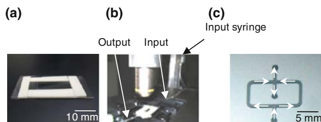
FIGURE 2. Microfluidic chip design (a) Cell reservoir used for static experiments and uniform flow experiments (30 mm × 10 mm). (b) Cell reservoir used for hydrostatic experiments. The input is set at different heights while the output is closed. (c) Silicone mold of the cross-junction channel. The channels are 50 μm deep × 500 μm wide. White arrows show the directions of the flow.
