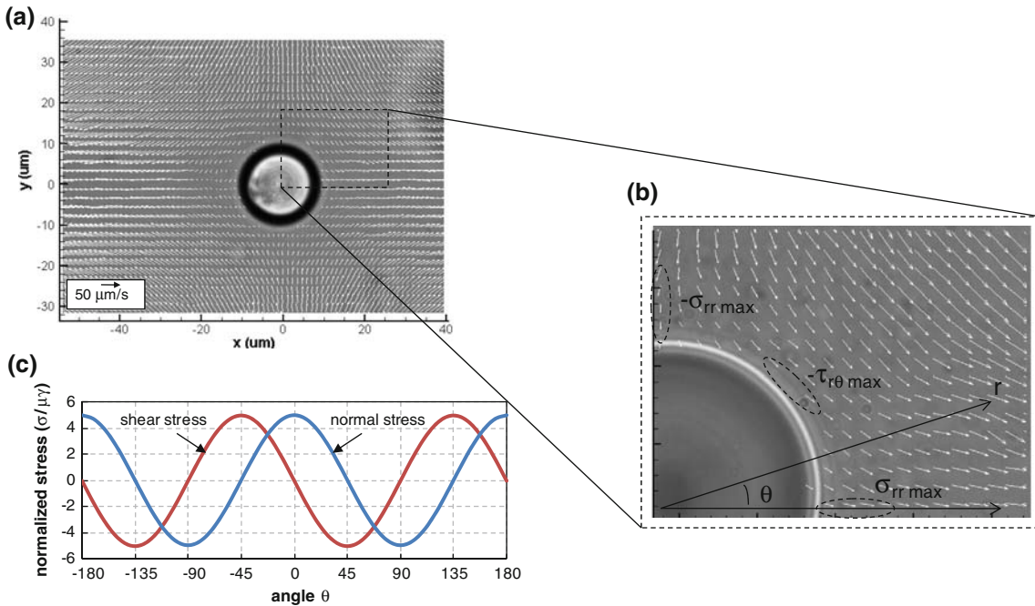
FIGURE 9. (a) The localized velocity field near a polystyrene sphere at the cross-flow region measured with \mu PIV. (b) Expanded view of the sphere quadrant and surrounding fluid with the location of the maximum shear, tension and compression stresses applied at the surface of the sphere. (c) The theoretical normalized shear, \tau_{r\theta} (red line) and normal, \sigma_{rr} (blue) stresses at the surface of a sphere ( r = a ).
