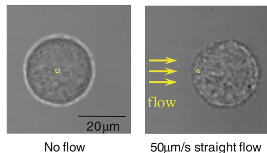
FIGURE 6. A 19.1 \mu\text{m} diameter chondroblast in static suspension (left). Visible cellular deformation of the cell due to an applied fluid shear stress induced by a straight channel flow (right). The circle represents the trap size (approximately 1.6 \mu\text{m} in diameter) and location.
