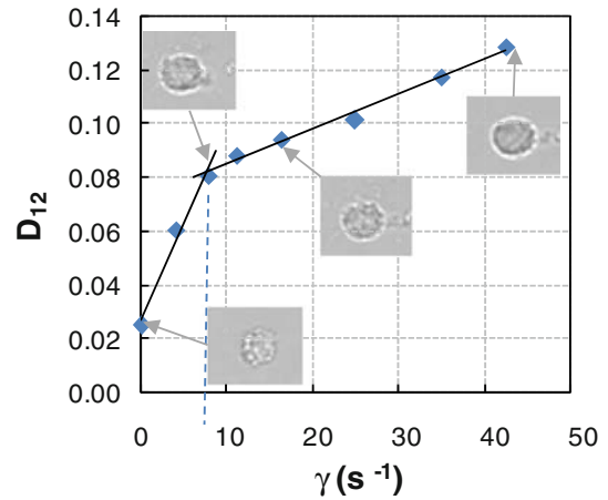
FIGURE 11. Deformation characteristics of a myoblast subjected to the cross junction extensional flow. Low extension rate ( < 7.8 \text{ s}^{-1} ) and high extension rate ( > 7.8 \text{ s}^{-1} ) deformation regimes are observed.
