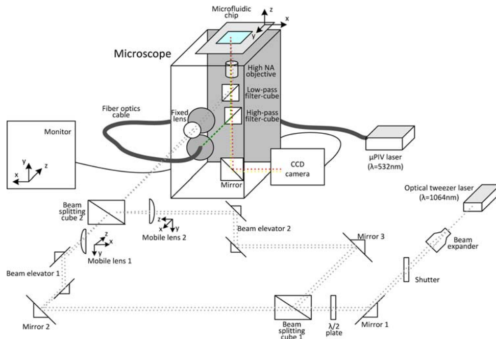
FIGURE 1. Schematic of the \mu PIVOT device and the current optical arrangement. The OT laser goes through different optical components including beam splitting cubes to allow the existence of two lasers of opposite polarization. The position of their focus point can be controlled independently using two mobile lenses that translate in any direction with automated control ( 0.1 \mu\text{m} resolution). Both traps can operate simultaneously or individually using shutters placed in the laser beams paths. Both of the OT lasers reunite through a second beam splitting cube before entering the microscope through an optical port. The \mu PIV lasers enter through a second port via an optical cable.
