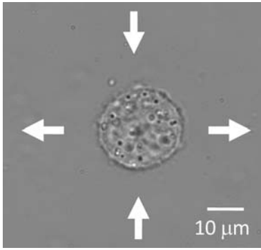
FIGURE 10. A living, 20 \mu\text{m} diameter osteoblastic optically trapped in the microfluidic cross-junction flow. The arrows are drawn to illustrate the flow direction.
