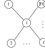
Fig. 10. Flow contention graph of flow i and |F_i| independent interferers.
