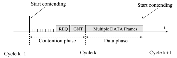
Fig. 1. Basic operations of S-CSMA
