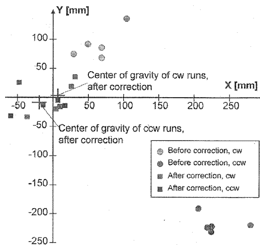
Fig. 11. Position errors after completion of the Bidirectional Square Path Experiment 4 \times 4 m). Before calibration: b = 340.00 mm, D_R/D_L = 1.00000 . After calibration: b = 336.17 mm, D_R/D_L = 1.00084 .
