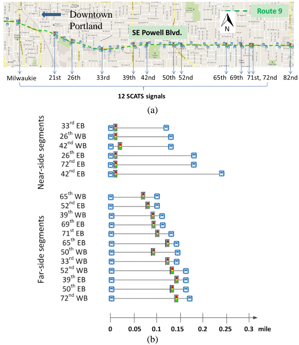
FIGURE 1 Study corridor and bus stop-to-stop segments.
