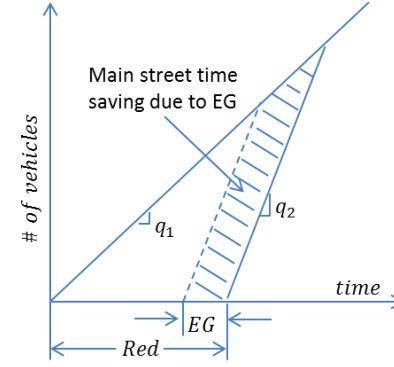
FIGURE 9 Illustration of major street time savings and side street delay.
