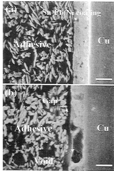
Fig.3 Interface microstructure of (a) as-joined and (b) heat-exposed for 300 h (SEM). The bars indicate 10 μm.
