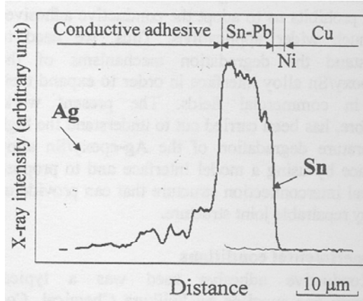
Fig.4 EPMA line analysis across interface heat-exposed for 300 h.
