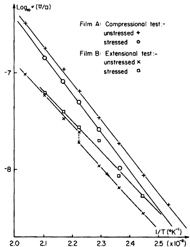
Fig. 3 Experimental DMTF strain effects: \delta E variation (Morris 1972d)
