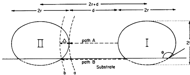
Fig. 1 The geometry of two ellipsoidal nanodots of eccentricity e = (1 - (t/r)^2)^{1/2} (Morris and Coutts 1977)
