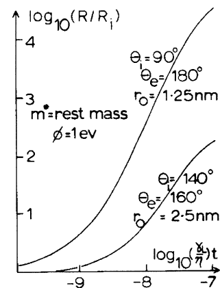
Fig. 4 DMTF R(t) model with adatom collection and surface self-diffusion (Morris 1975a)
