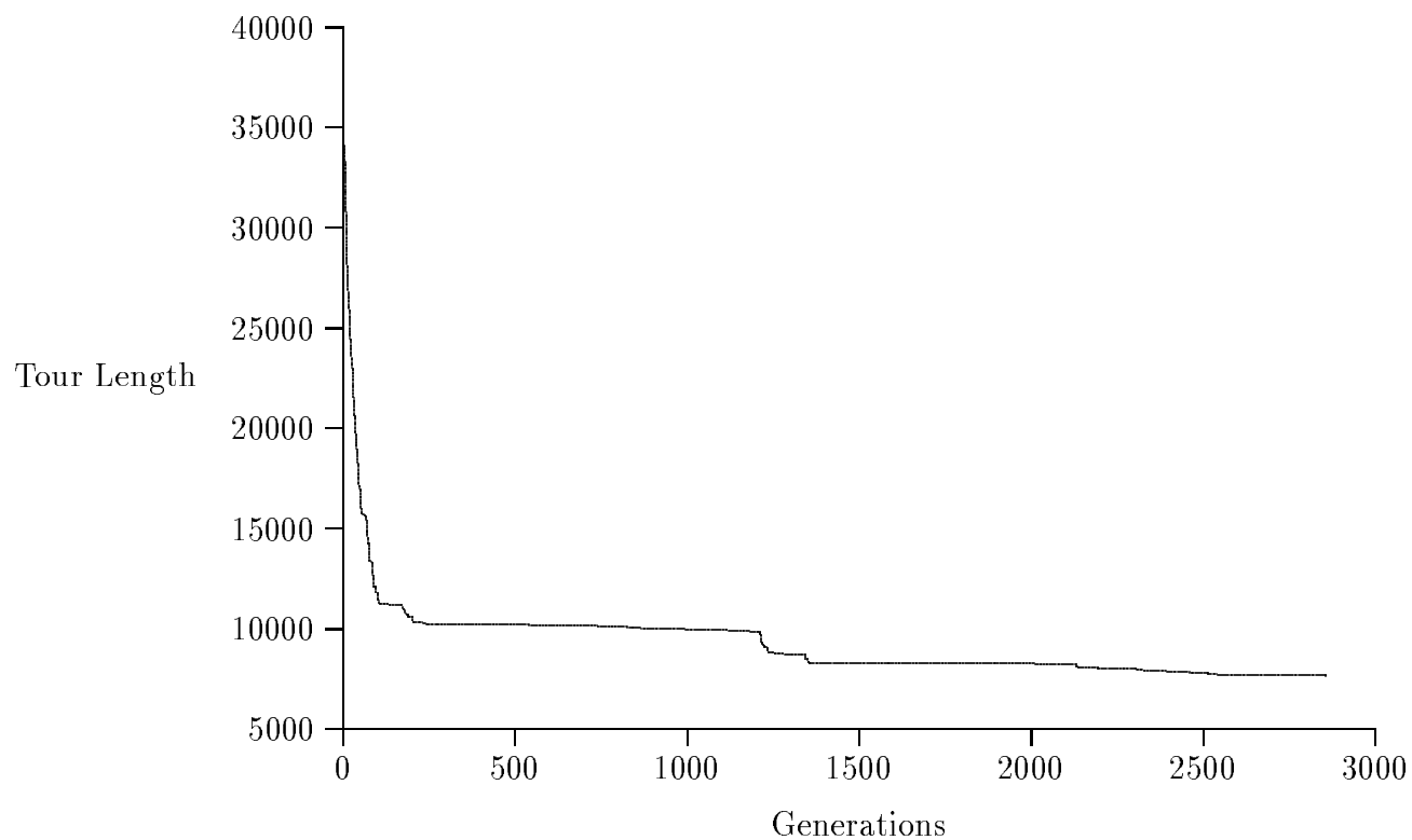
Figure 1: Typical (1,30) ES run result for the 80-city TSP using a single, self-adapted mutation operator. The best tour length found was 7638.1 miles. The best tour was found in generation 2857.
