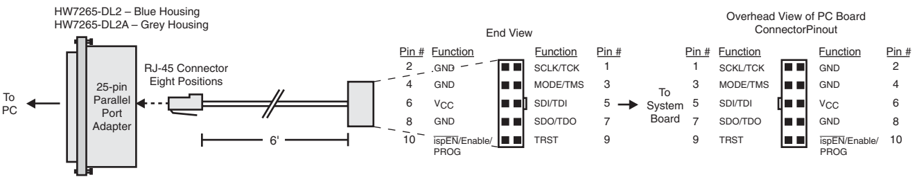
Figure 4. ispDOWNLOAD Cable In-System Programming Interface for the PC (HW7265-DL2 or HW7265-DL2A)
