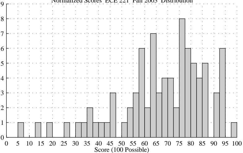
Normalized Scores ECE 221 Fall 2003 Distribution
