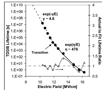
Figure 5. Long-term TDDB measured on the Final process flow shows a change in the acceleration slope at ~12MV/cm.
