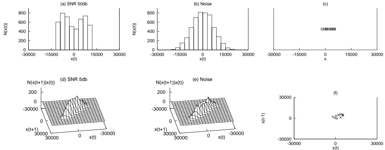
Figure 1: Histograms for detection: (a) A 20 bin histogram of a 5000 point sample of the target signal at 50 db SNR. (b) A 20 bin histogram of a 5000 point sample of the background noise. (c) A test sequence of ten observations. (d) A 20 \times 20 bin histogram of a 5000 point sample of the target signal at 5db SNR. (e) A 20 \times 20 bin histogram of a 5000 point sample of the background noise. (f) A test sequence of ten observations.
