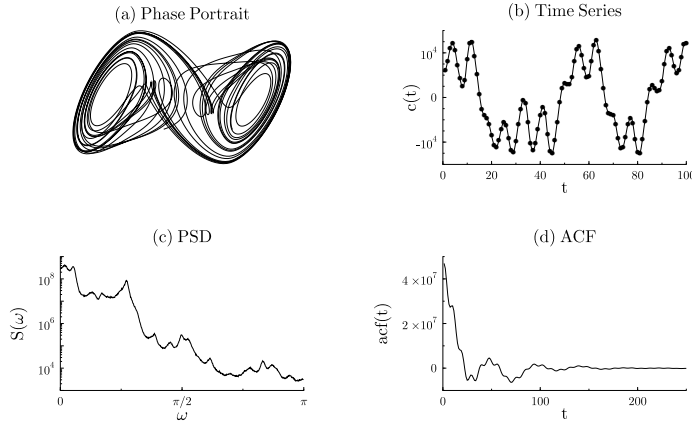
Figure 2: A strange (or chaotic) attractor. (a): A phase portrait of the Double Scroll system. (b): A scalar time series of the observable c(t) . (c): Fourier power spectrum of the observable. (d) The autocorrelation function.
