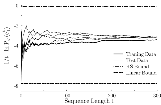
Figure 3: Average Log-Likelihood. A curve for the training data used to fit the 30 state model with 5 th order AR outputs and curves for four randomly selected realizations of the noise free signal c_1^{300} are plotted.
