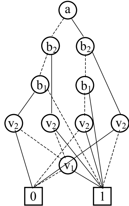
Fig. 12. The BEMDD for MVR F(A,B)
