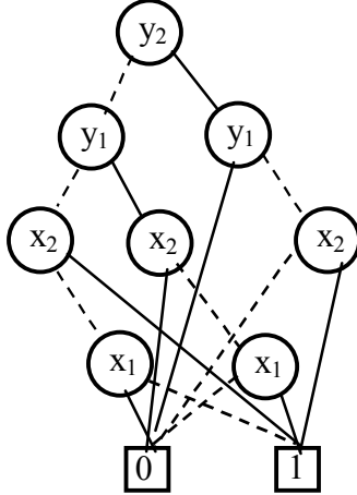
Fig. 4. The BDD for the given set of subsets
