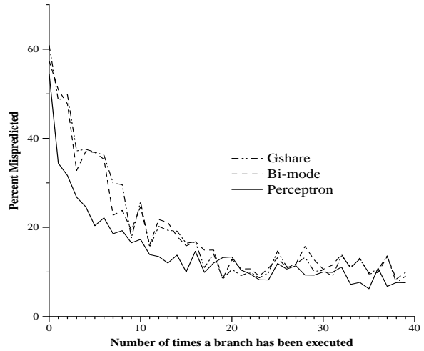
Figure 6: Average Training Times for gcc . The x axis is the number of times a branch has been executed. The y -axis is the average, over all branches in the program, of 1 if the branch was mispredicted, 0 otherwise. Over time, this statistic tracks how quickly each predictor learns. The perceptron predictor achieves greater accuracy earlier than the other two methods.
